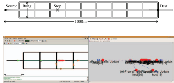
Fig. 1. Baseline scenario used in the evaluation: a single trunk road is connected to two slower parallel roads by a number of rungs. Concept and representations in the road traffic and network traffic simulators.
