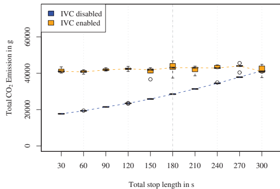
(b) influence of stop length on emissions; 100 m rungs
