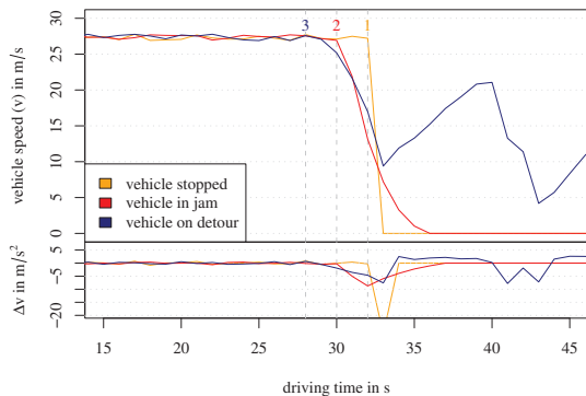
Fig. 2. Impact of route choice on vehicle speed and acceleration profile
